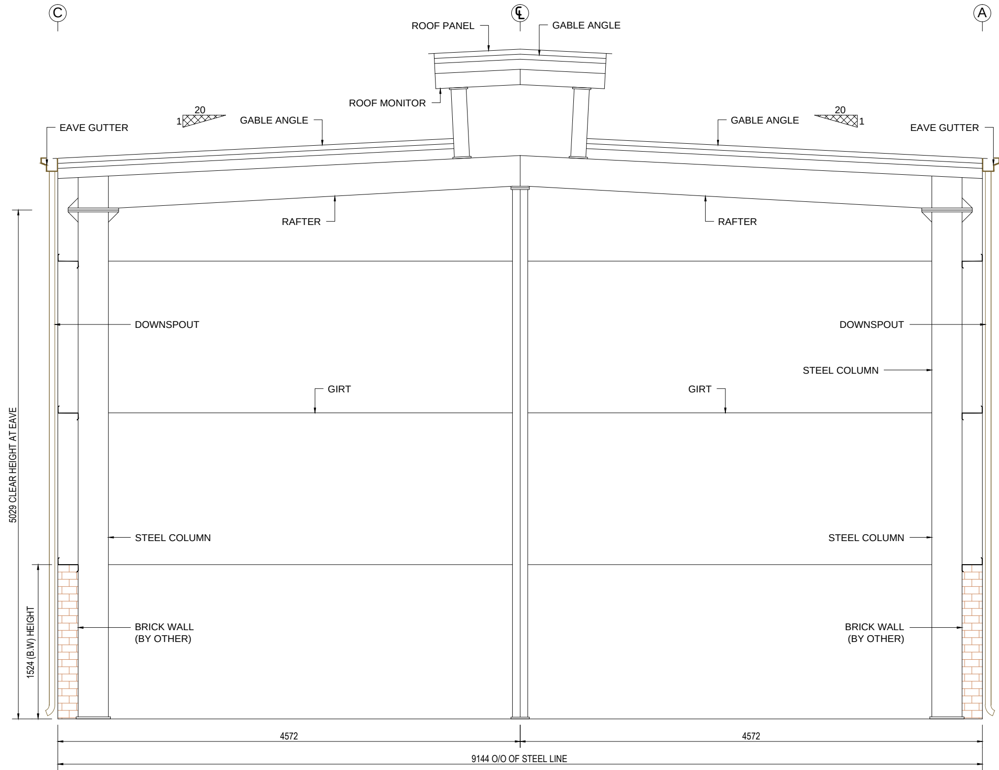
END WALL FRAMING @ GRID-3
